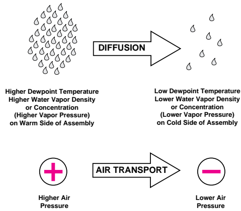
Figure 1 Water Vapor Movement
