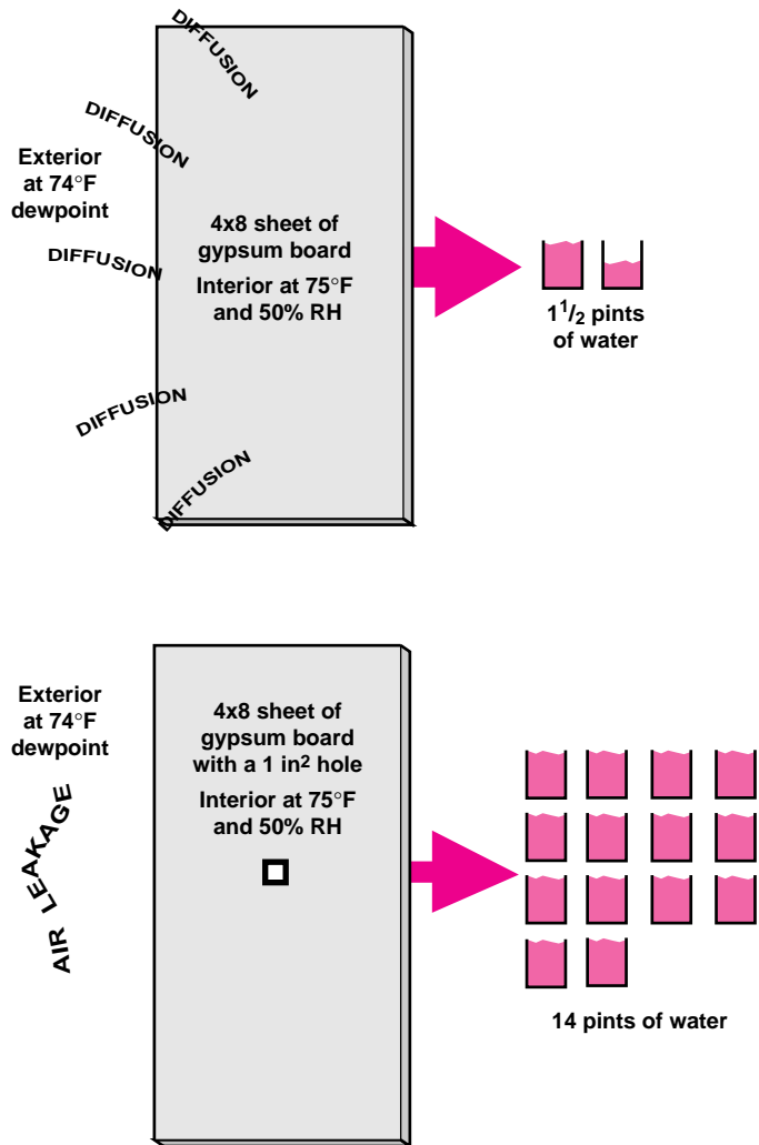
Figure 4 Diffusion vs. Air Leakage
