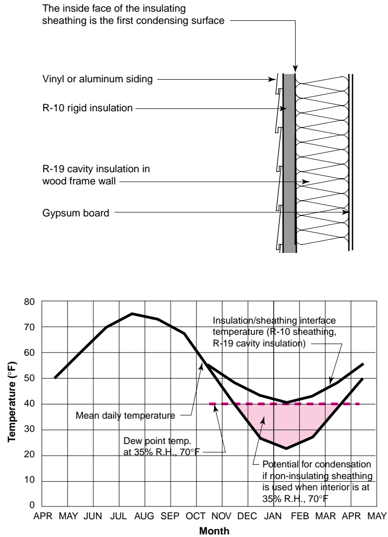
Figure 11 Potential for Condensation in a Wood Frame Wall Cavity Without an Interior Vapor Diffusion Retarder in Chicago, Illinois (Cold Climate)
