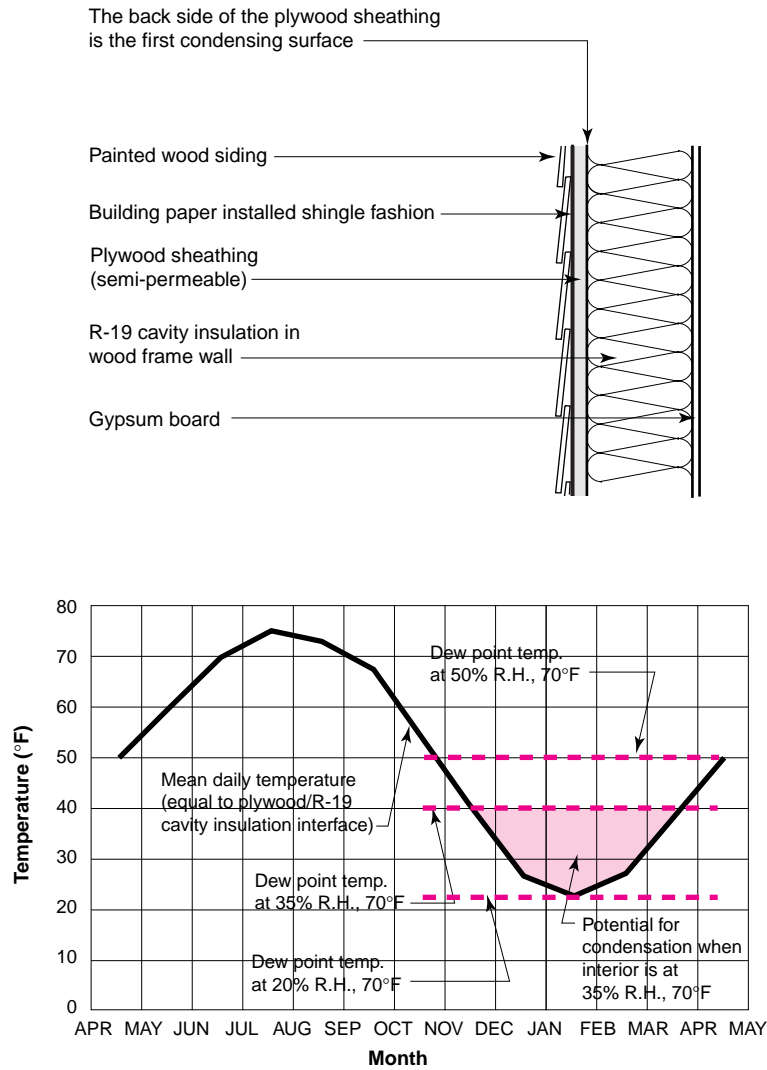
Figure 10 Potential for Condensation in a Wood Frame Wall Cavity in Chicago, Illinois (Cold Climate)
