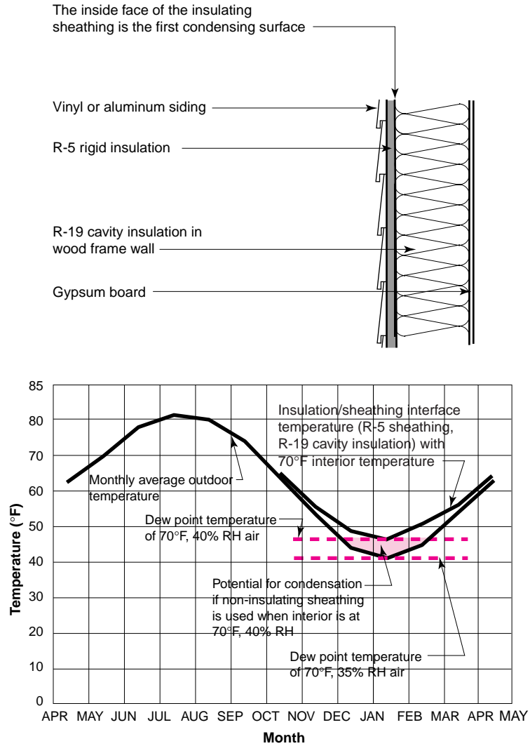
Figure 12 Potential for Condensation in Tupelo, Mississippi (Mixed-Humid Climate)
