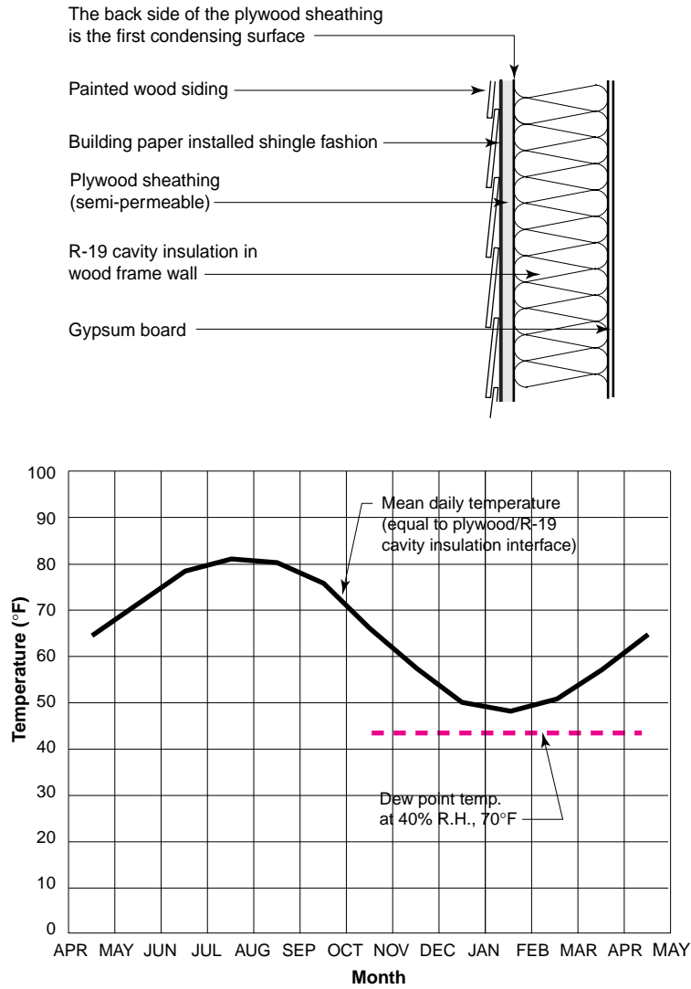
Figure 13 Potential for Condensation in Charleston, South Carolina (Hot-Humid Climate)
